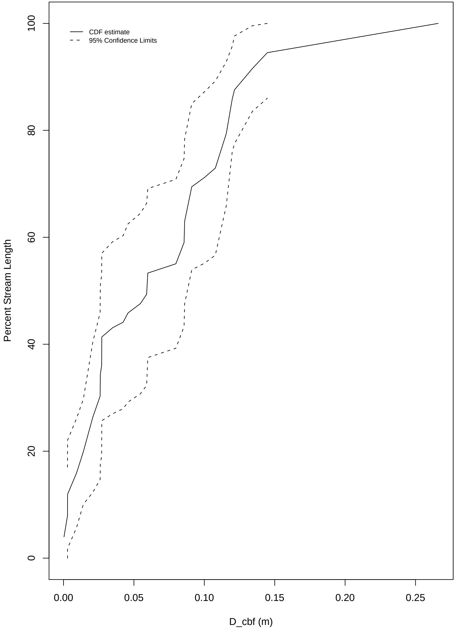
SWIM Distribution
